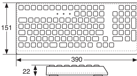
TT-108 Dimensions in [mm]
