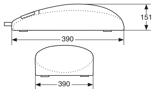
KM-25-SI Dimensions in [mm]
